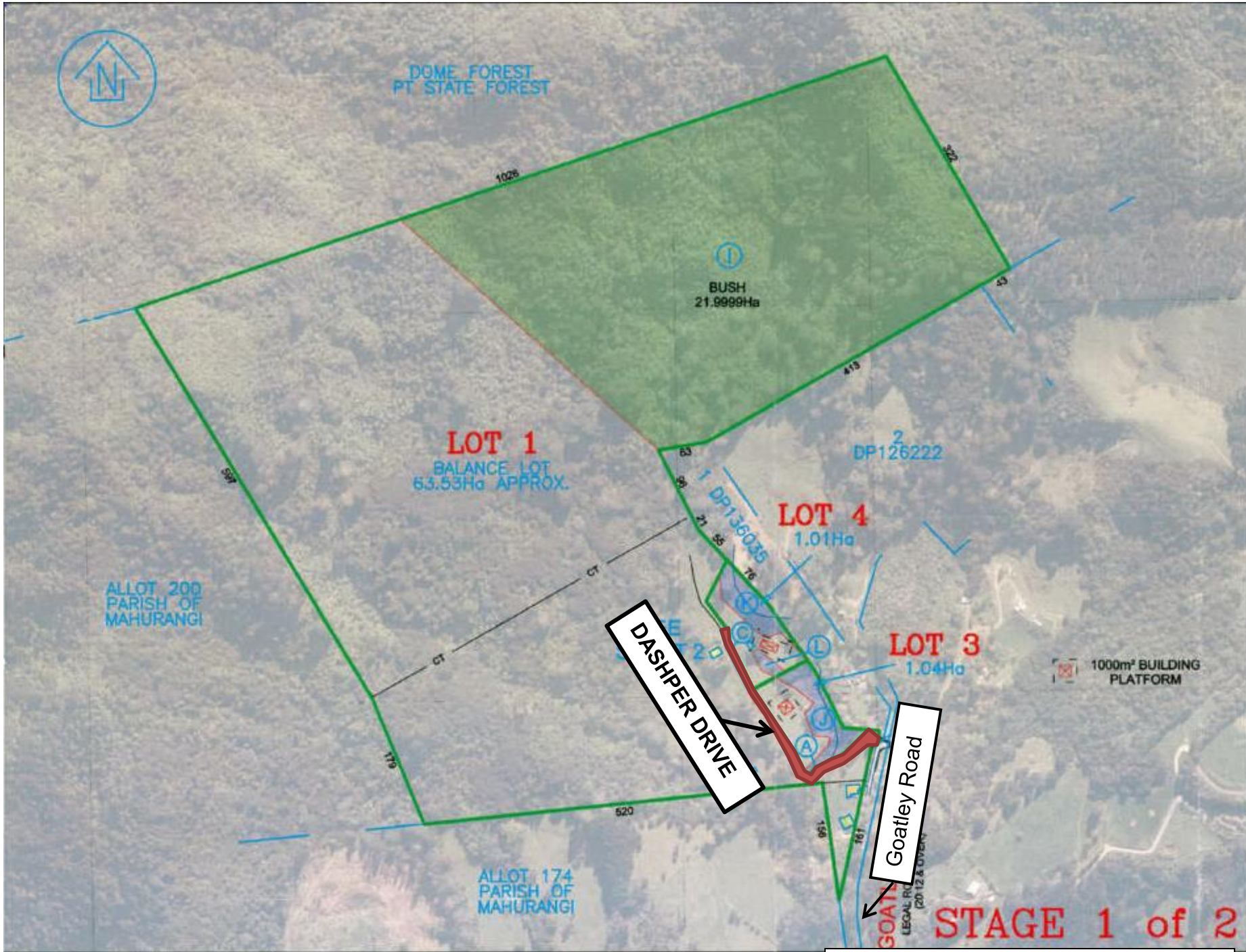
Dashper Drive Scheme Plan
