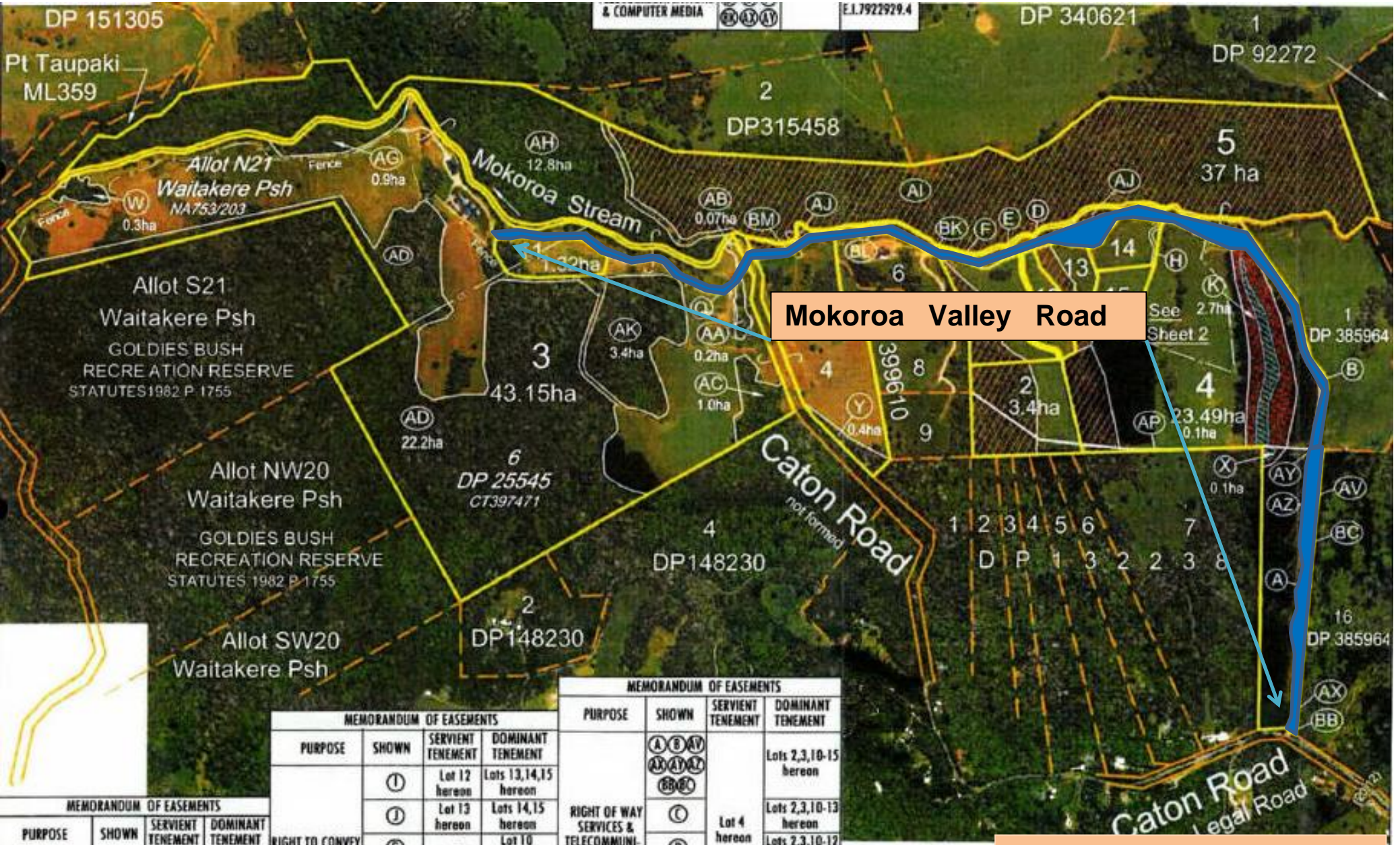
Mokoroa Valley Road Scheme Plan
