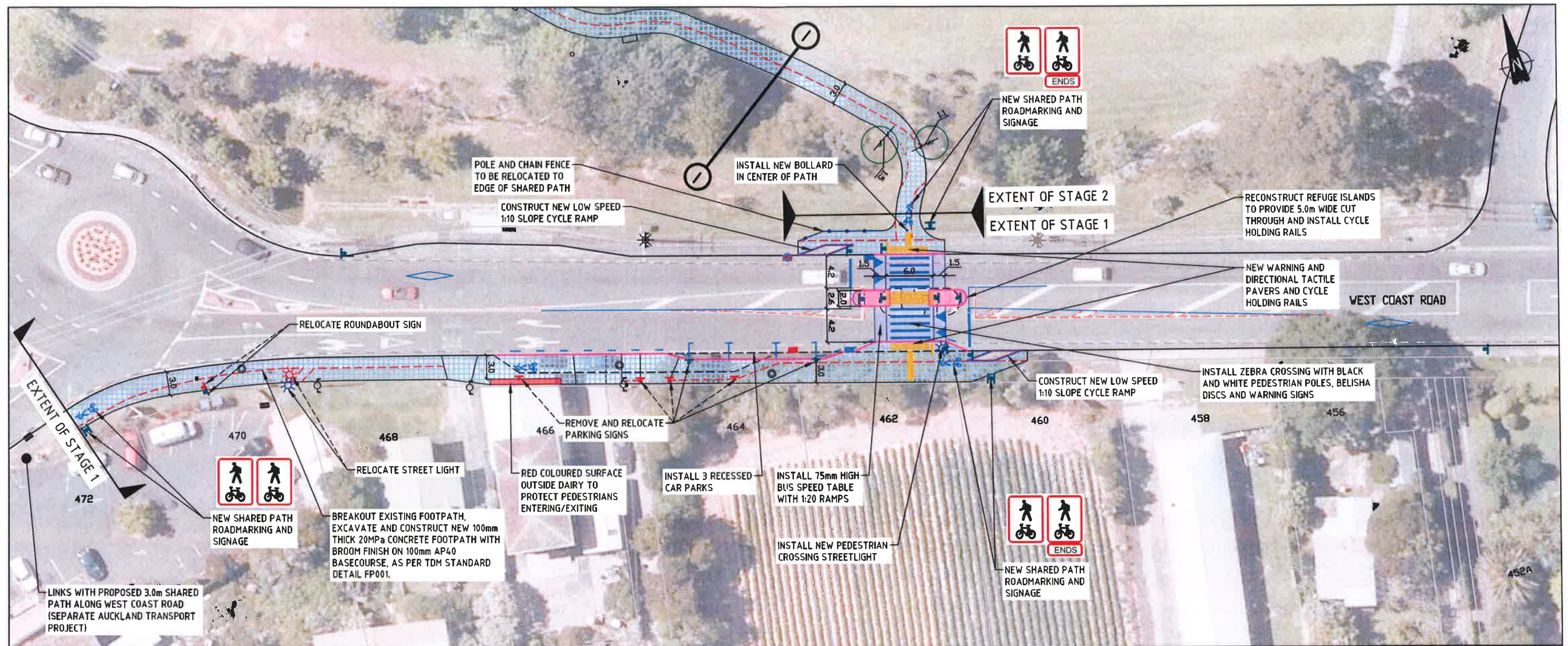
ROUTE LAYOUT PLAN SCALE 1:250 (A1), 1:500 (A3)
