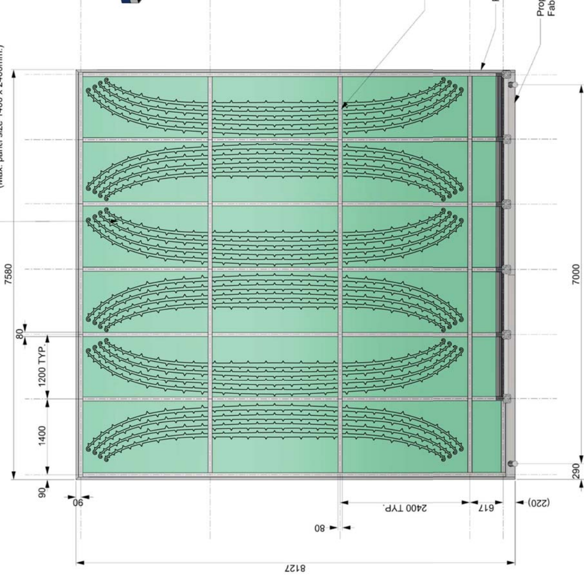
Ceiling Plan Scale 1:50
