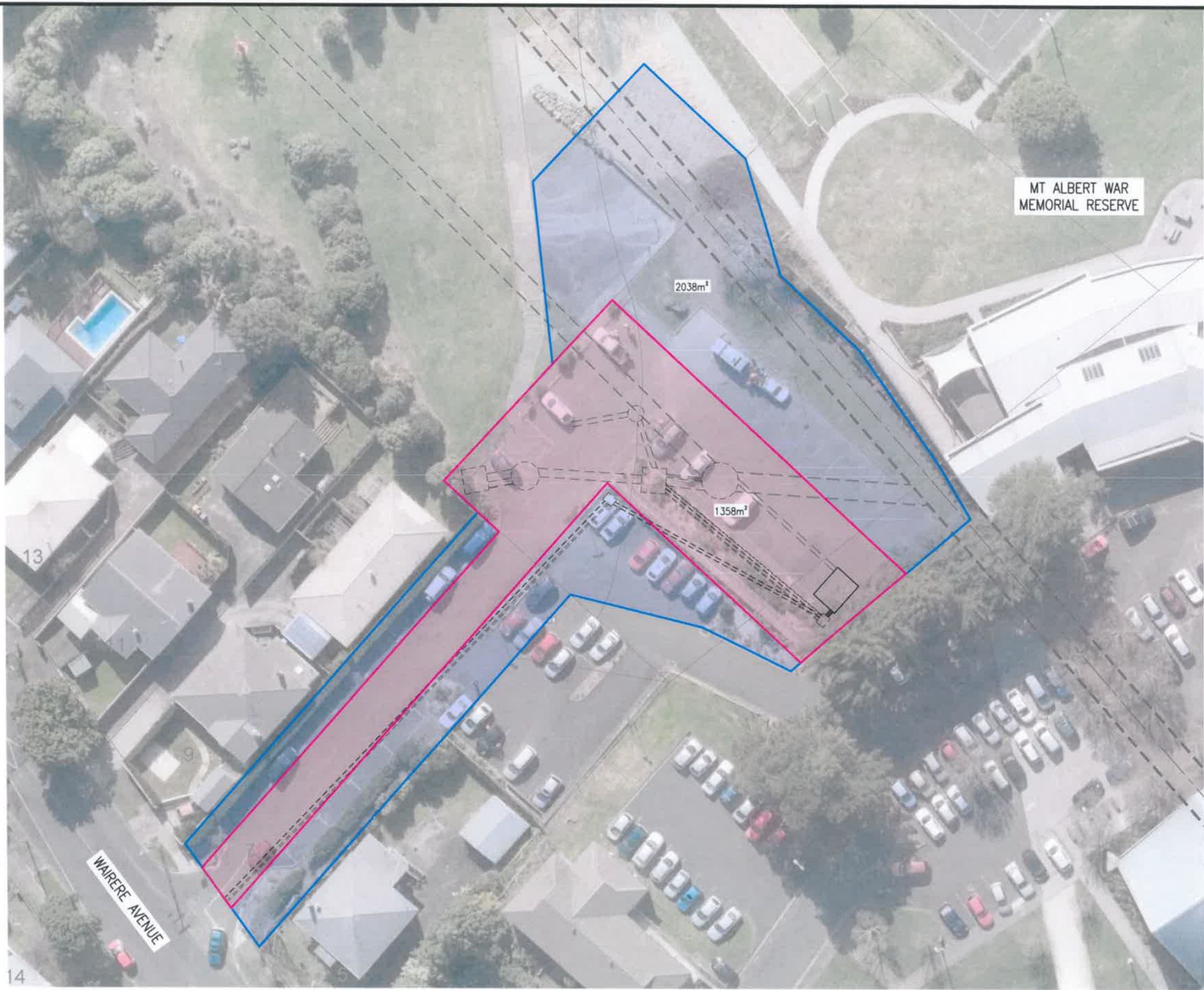
PLAN SCALE 1:250 (A1)
