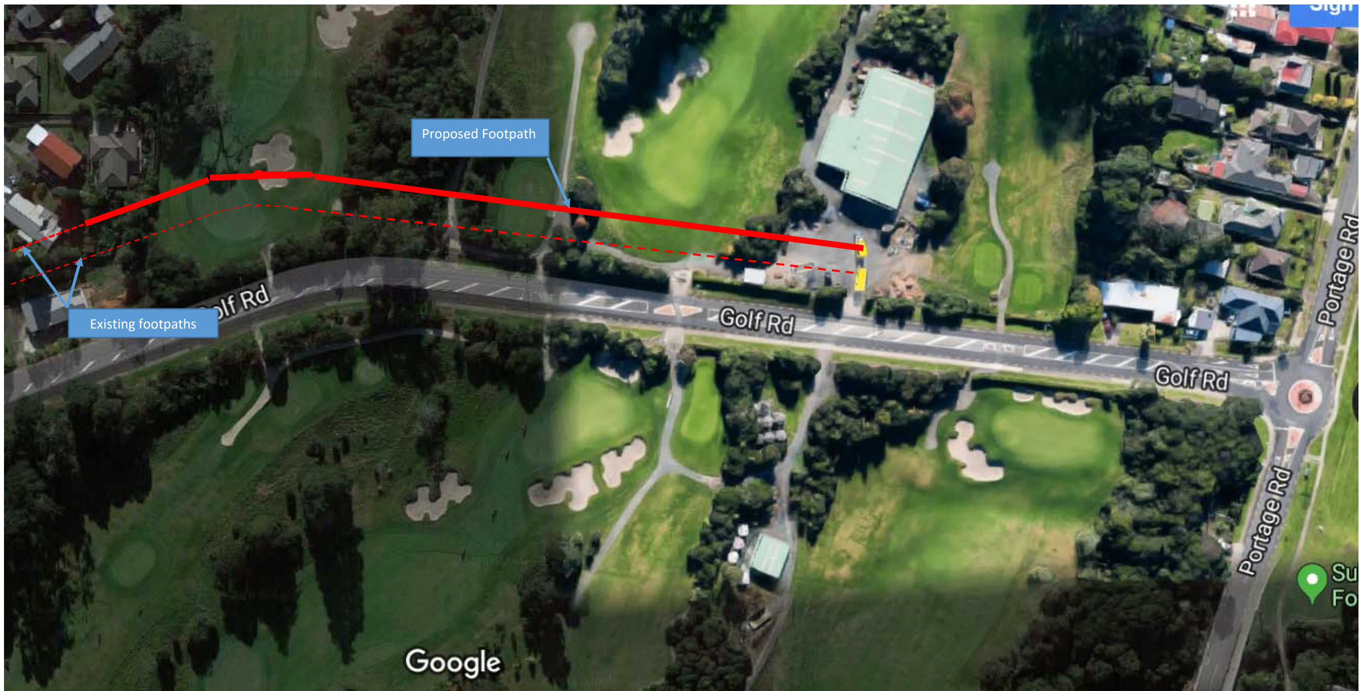
OPTION 1 – 1.8m FOOTPATH
