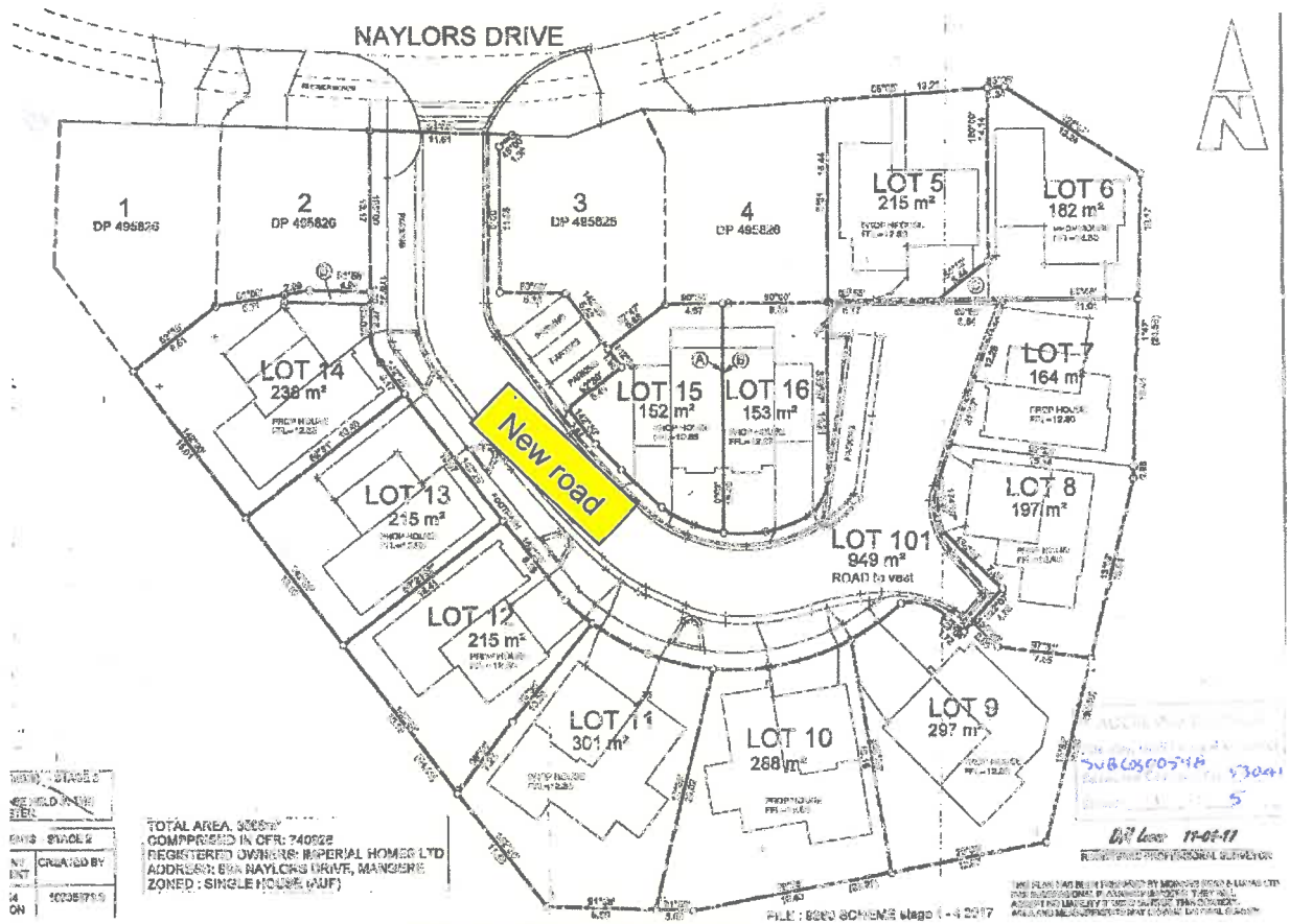
Figure 2: Scheme Plan; 89A Naylor's Drive, Mangere.
