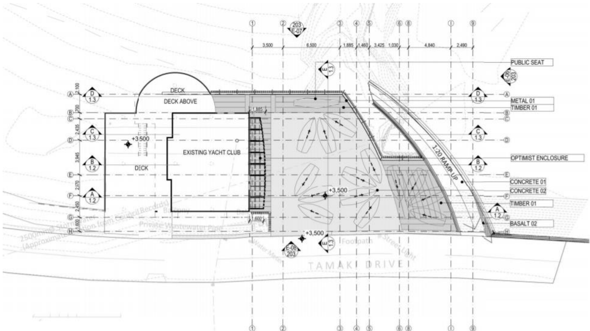
1. MAIN DECK LEVEL 1:200
