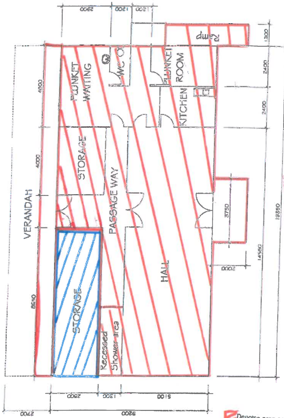
RIVERHEAD WAR MEMORIAL PAVILION - FLOOR LAYOUT. 1:100.
