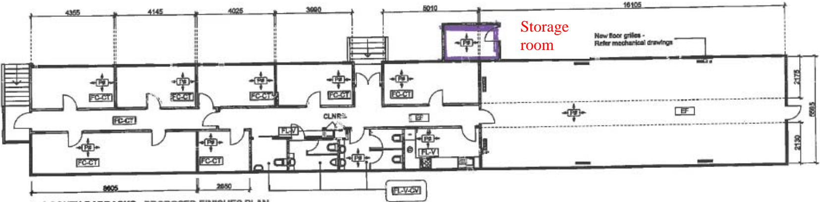
A13 SOUTH BARRACKS - PROPOSED FINISHES PLAN
