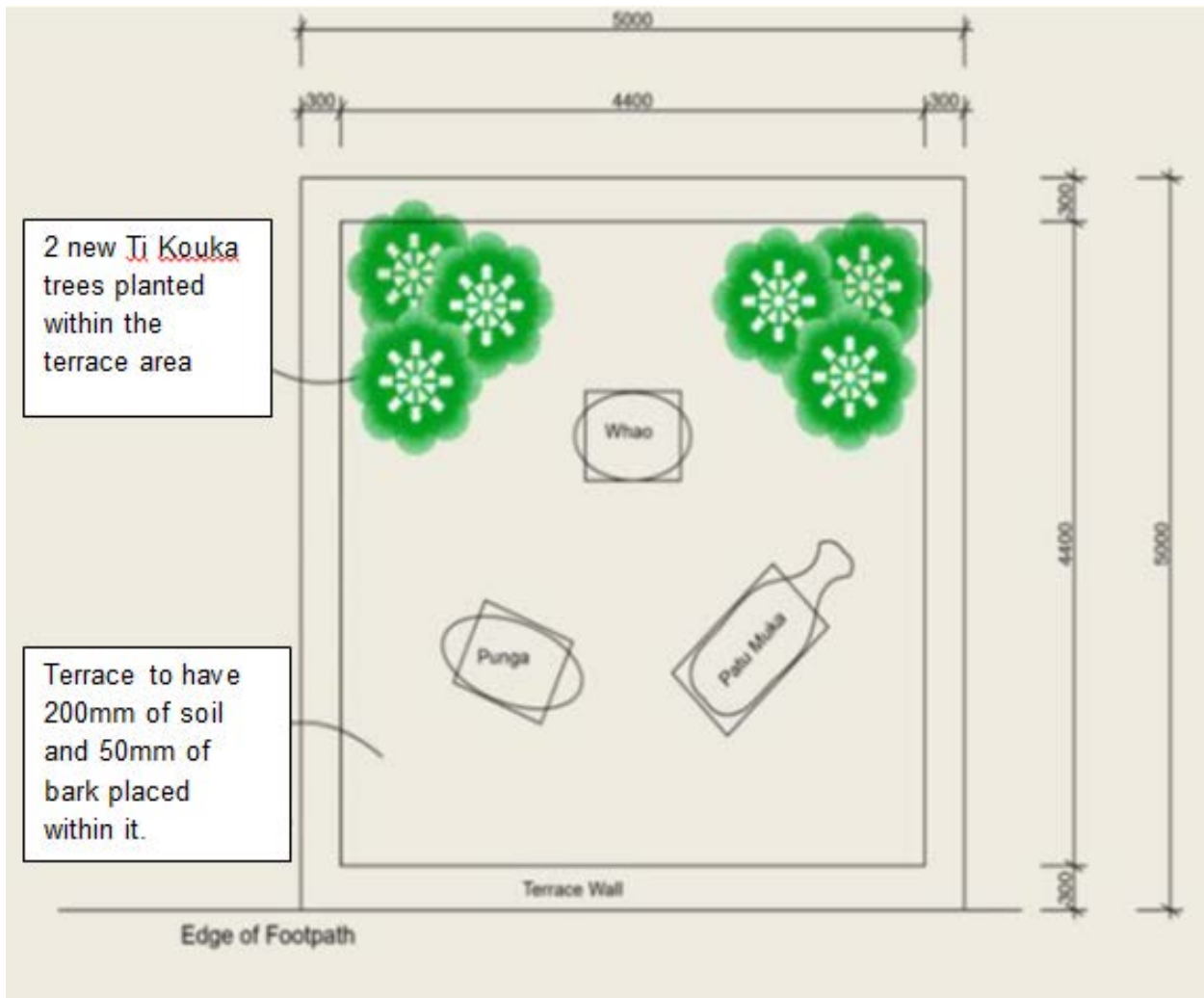
Figure 2 – Detailed plan of artwork area
