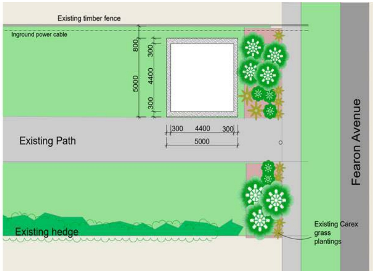
Figure 4 – Dimensions of proposed artwork area.
